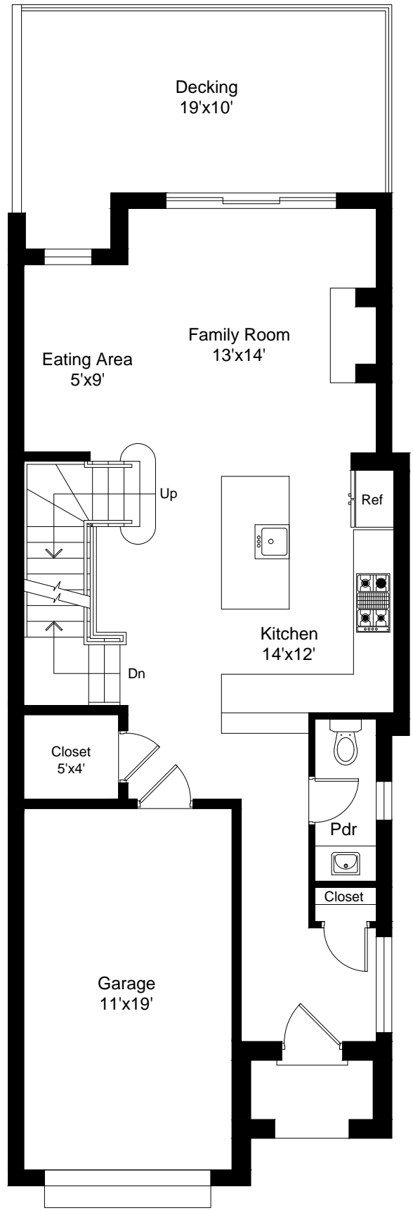
FIRST FLOOR
