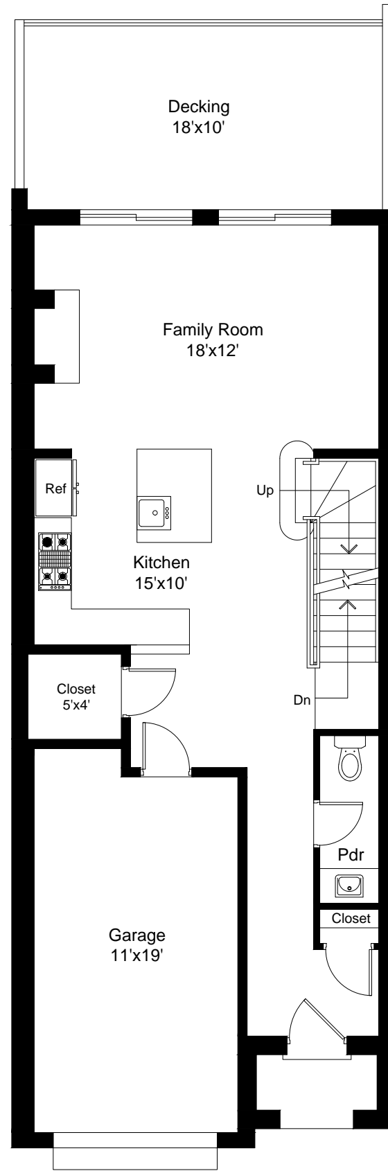
FIRST FLOOR
